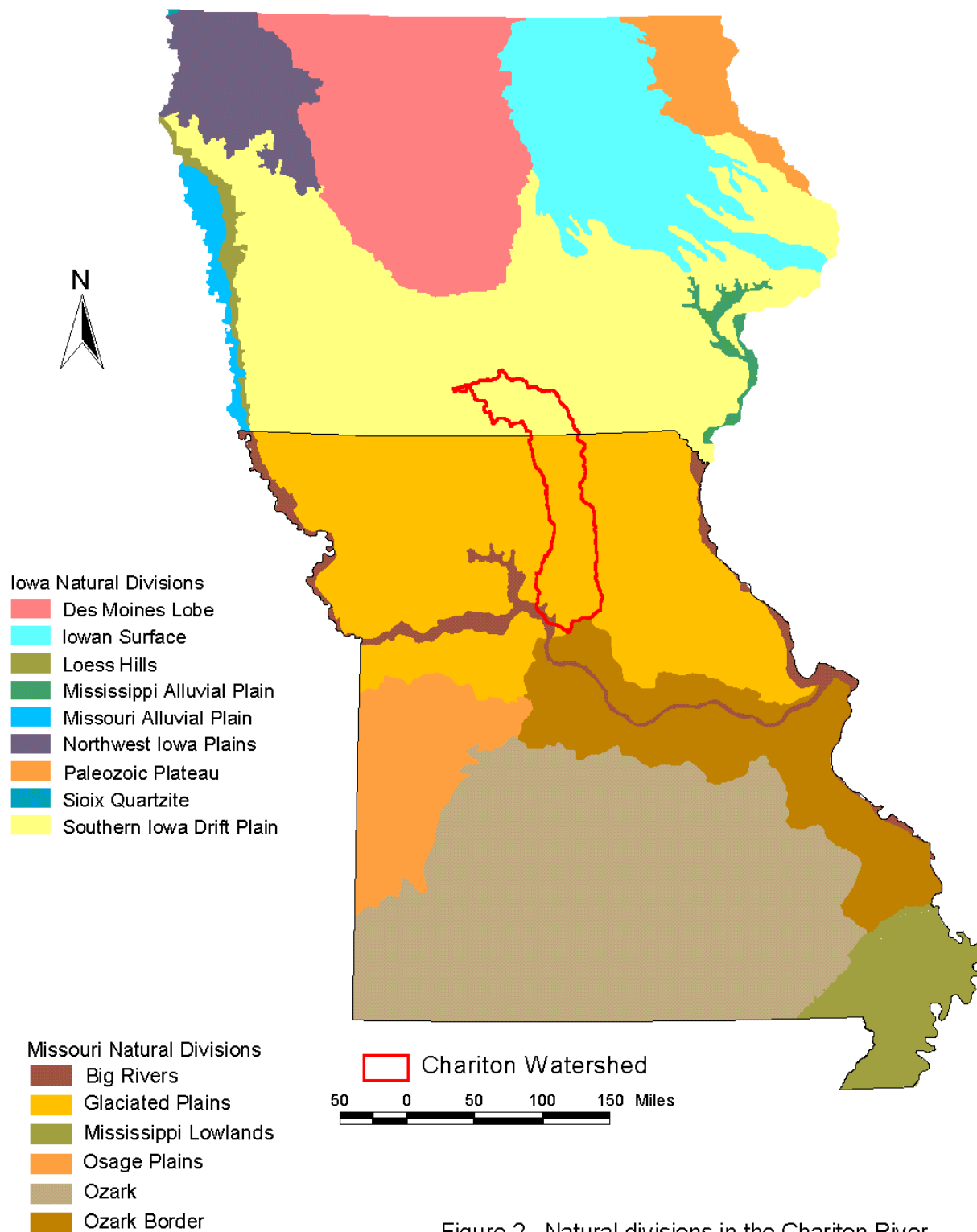
Figure 2. Natural divisions in the Chariton River watershed, in Missouri and Iowa.
